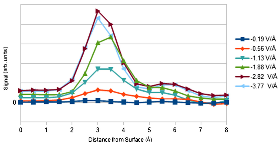
Figure 6 Integrated contrast line scan vs. electric field. Two contrast features due to EDL structure are found at 3 and 6 \text{ Å} . Peak maxima, at 3 \text{ Å} , scale near-linearly with cesium packing density. The gold surface is located at the origin. MD-determined results are shown.
