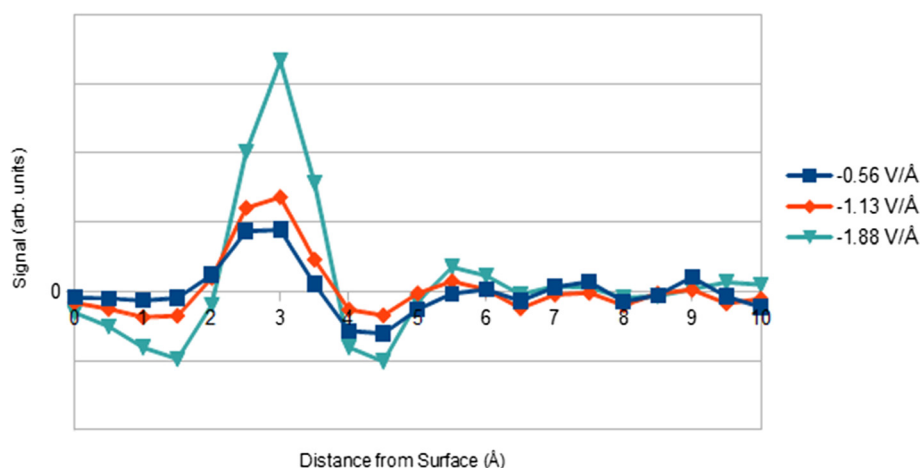
Figure 7 Integrated contrast line scan vs. electric field when cesium ions are substituted with lithium ions. Contrast fringes form, and the structure-contrast relationship becomes more difficult to evaluate. The gold surface is located at the origin.
